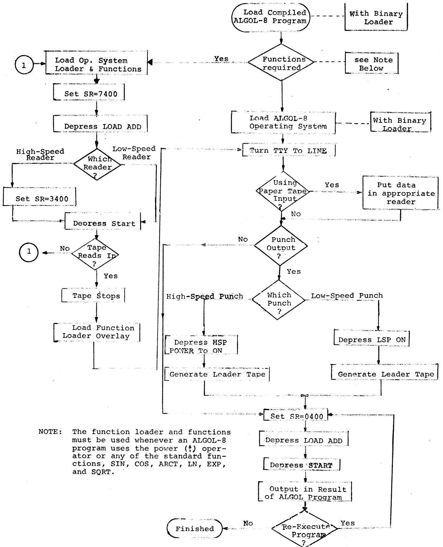
Figure 8-2 Running an ALGOL-8 Program.
